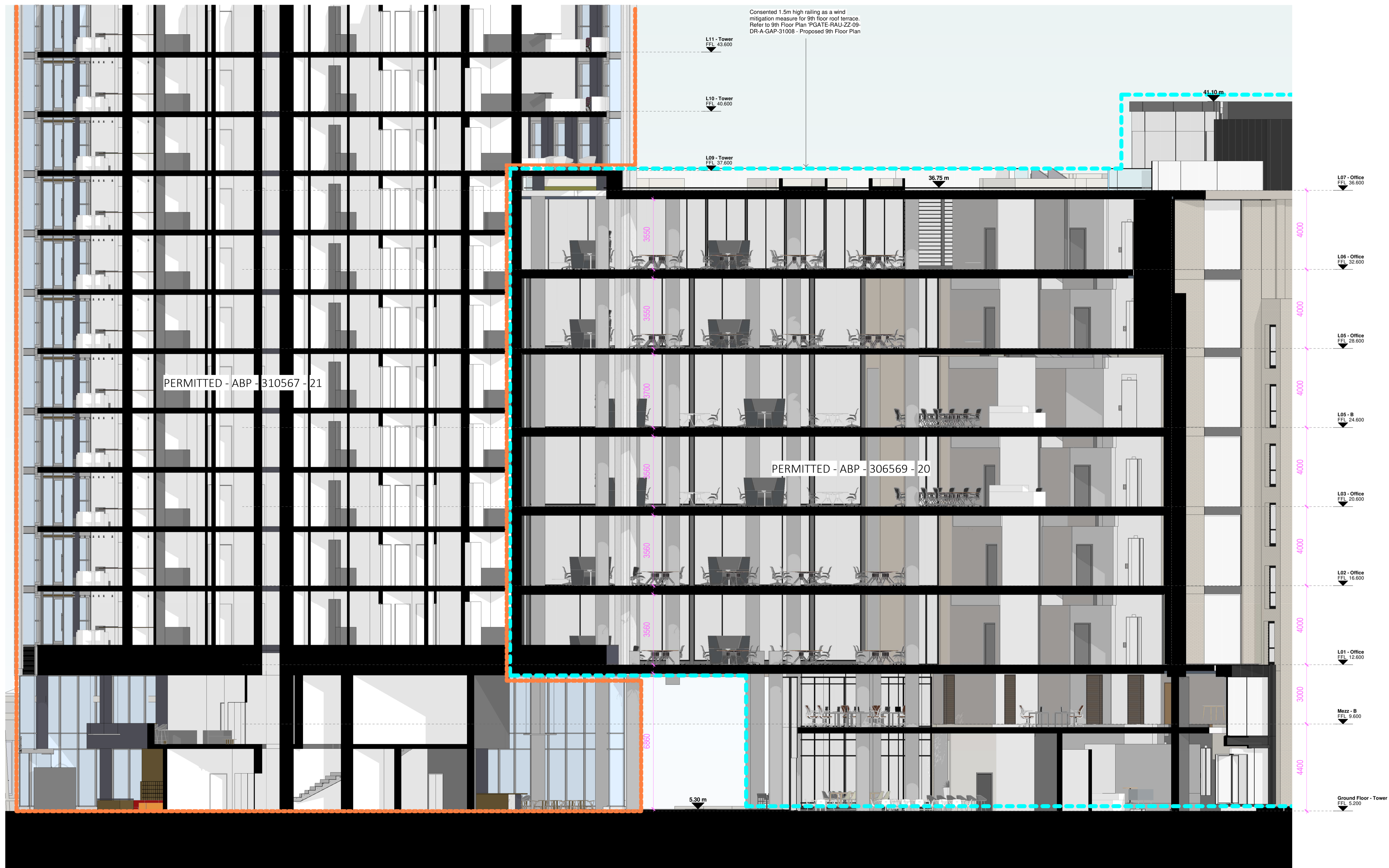
Permitted Section BB 1 : 100
